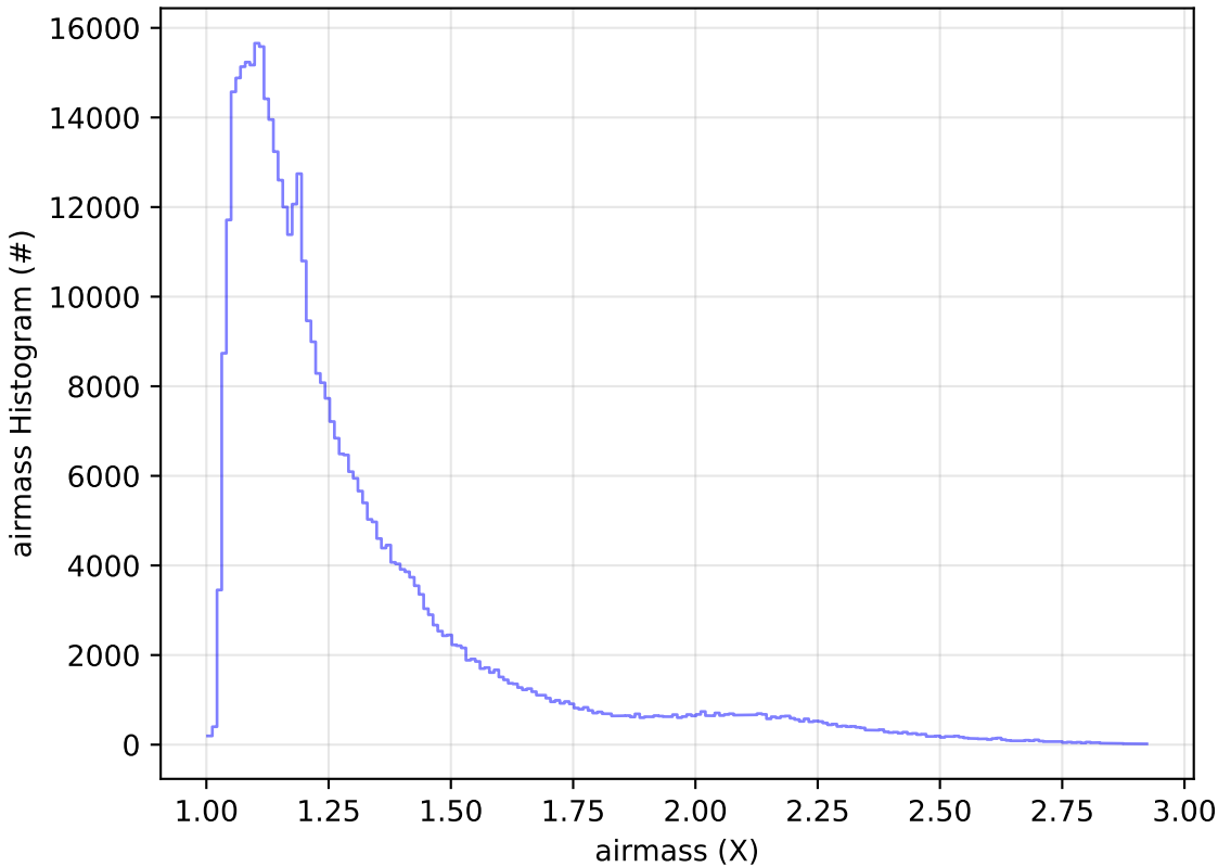
telescope_jerk_v3.5_10yrs WFD i band: airmass Histogram
