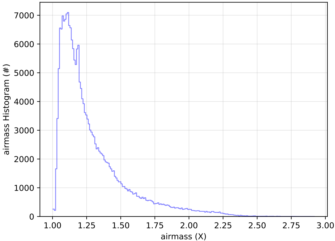
telescope_jerk_v3.5_10yrs WFD g band: airmass Histogram
