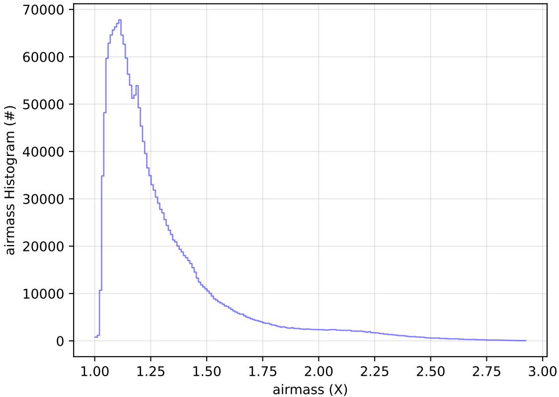
telescope_jerk_v3.5_10yrs WFD all bands: airmass Histogram
