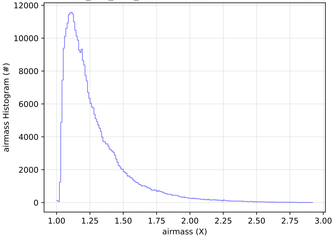
telescope_jerk_v3.5_10yrs All sky y band: airmass Histogram
