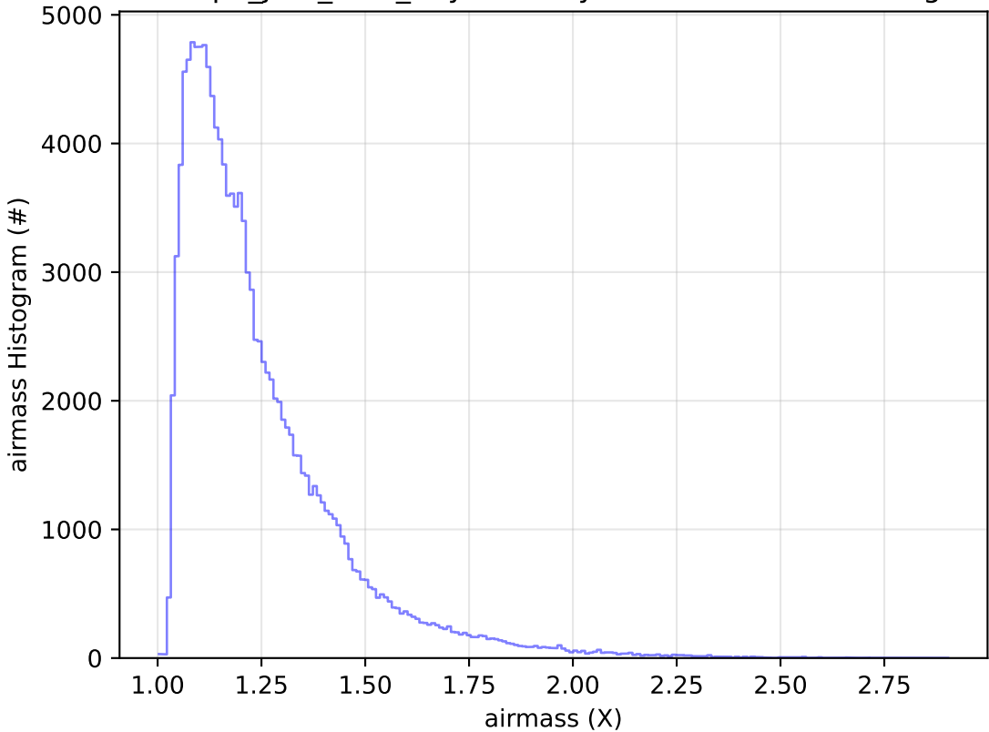
telescope_jerk_v3.5_10yrs All sky u band: airmass Histogram
