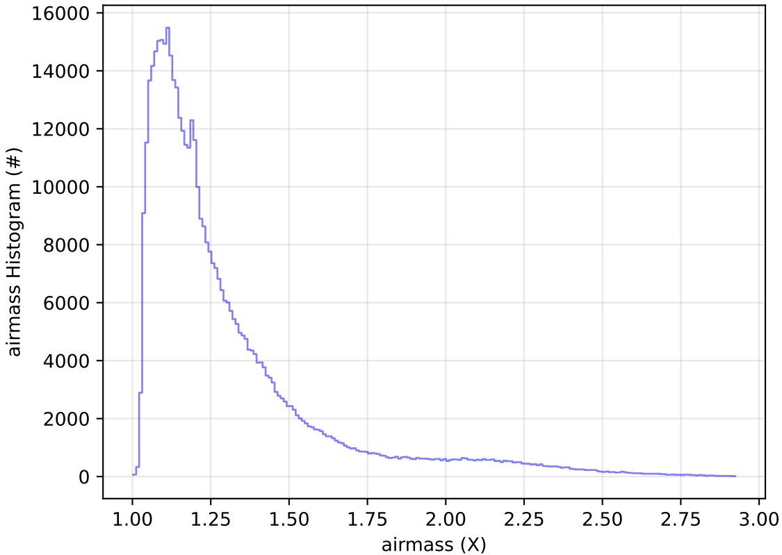
telescope_jerk_v3.5_10yrs All sky r band: airmass Histogram
