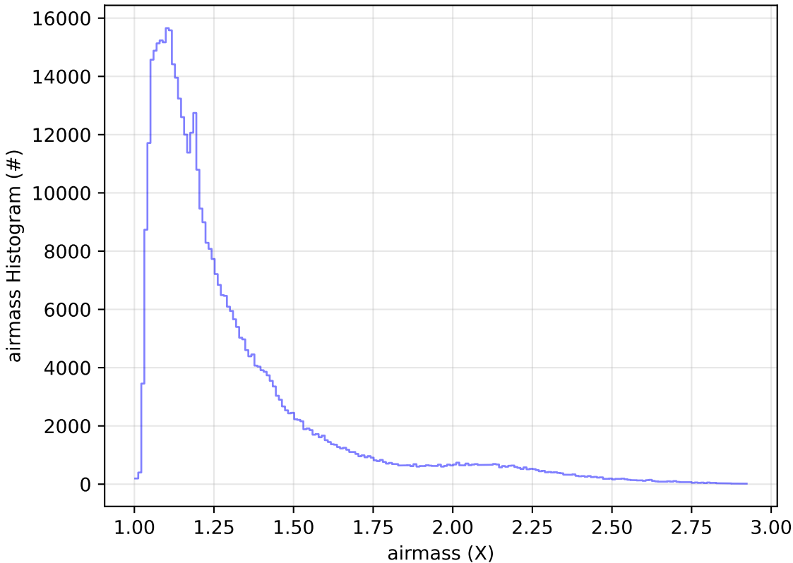
telescope_jerk_v3.5_10yrs All sky i band: airmass Histogram
