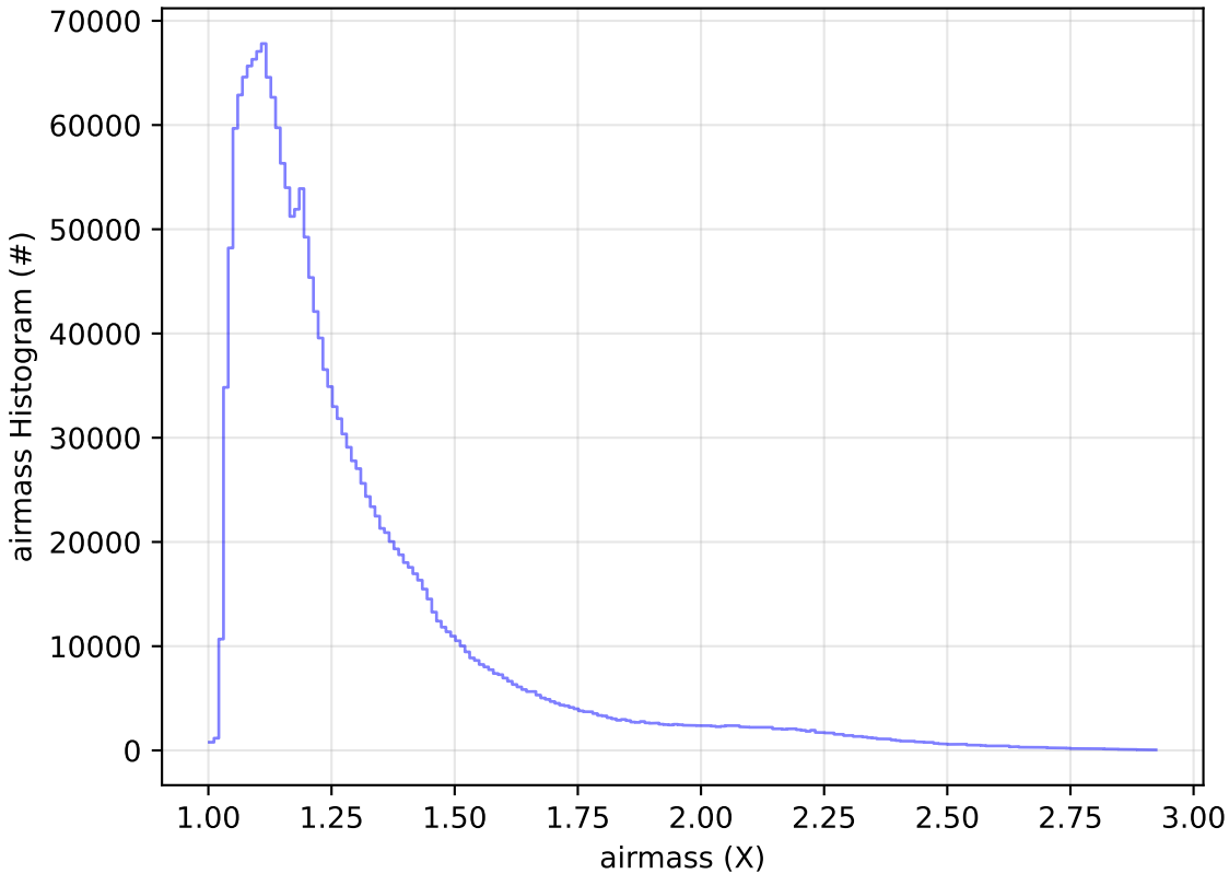
telescope_jerk_v3.5_10yrs All sky all bands: airmass Histogram
