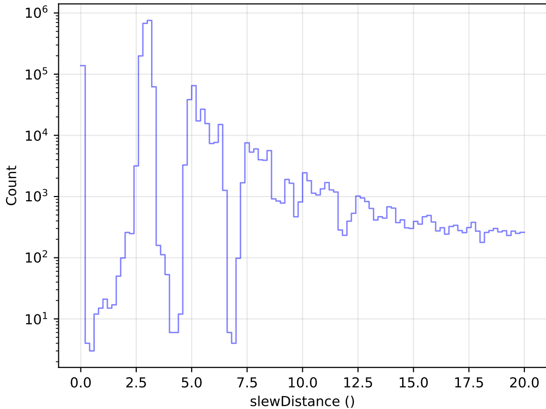
telescope_jerk_v3.5_10yrs All visits: Zoom Slew Distance Histogram
