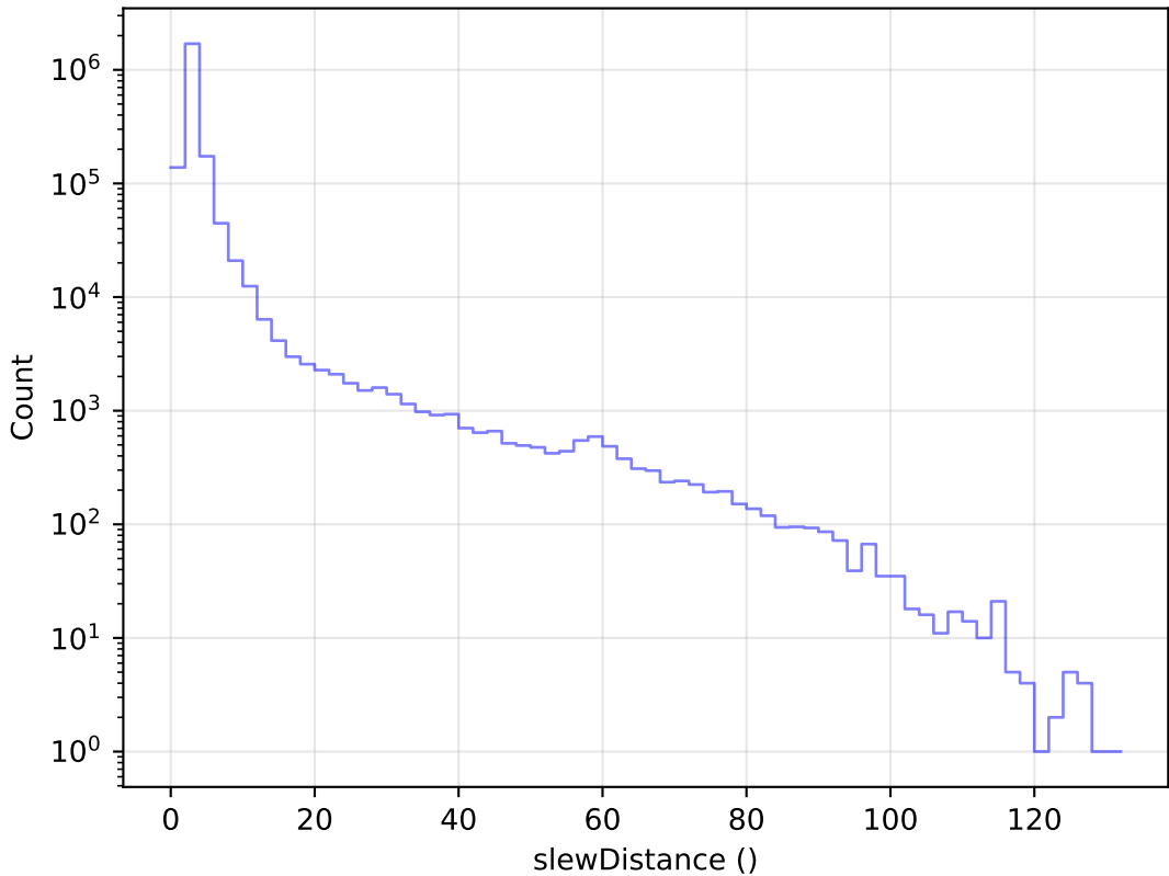
telescope_jerk_v3.5_10yrs All visits: Slew Distance Histogram
