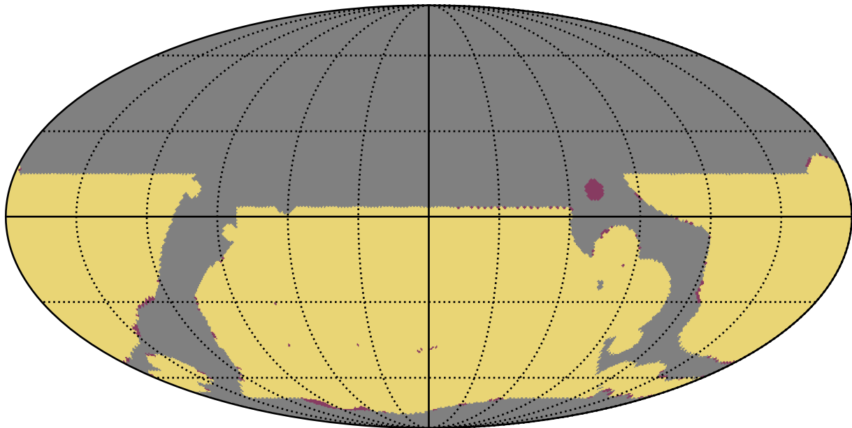
telescope_jerk_v3.5_10yrs WFD: RapidRevisits
