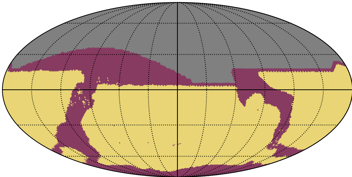
telescope_jerk_v3.5_10yrs All sky: RapidRevisits
