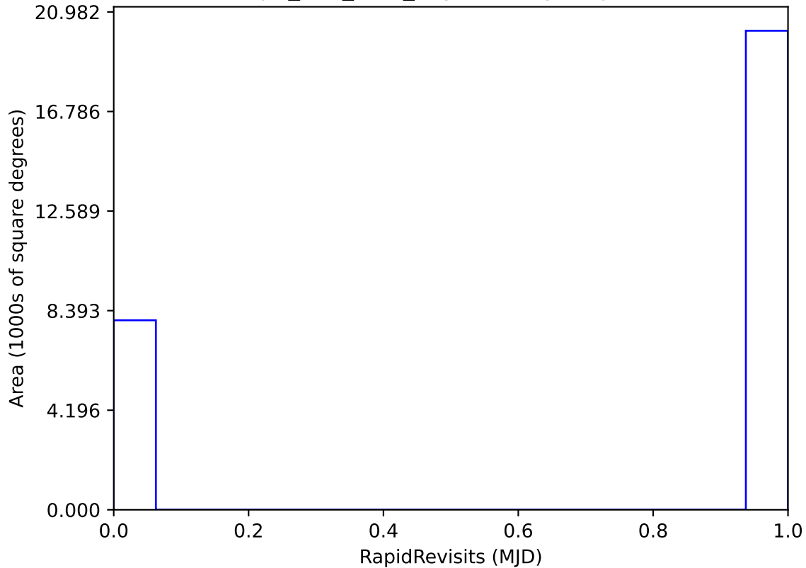
telescope_jerk_v3.5_10yrs All sky: RapidRevisits
