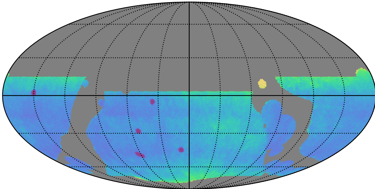
telescope_jerk_v3.5_10yrs WFD: Proper Motion Uncert @ 24.0
