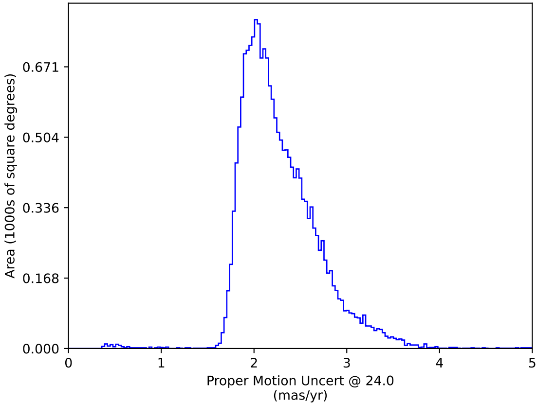
telescope_jerk_v3.5_10yrs WFD: Proper Motion Uncert @ 24.0
