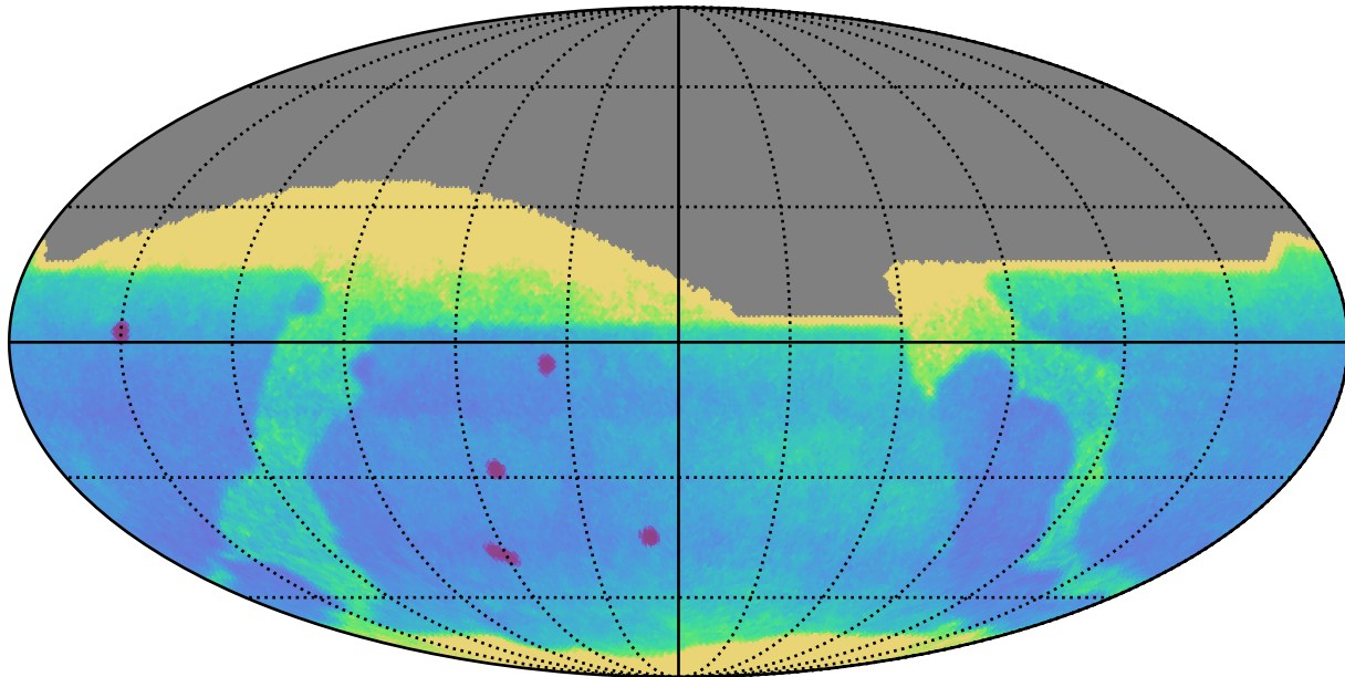
telescope_jerk_v3.5_10yrs All sky: Proper Motion Uncert @ 24.0
