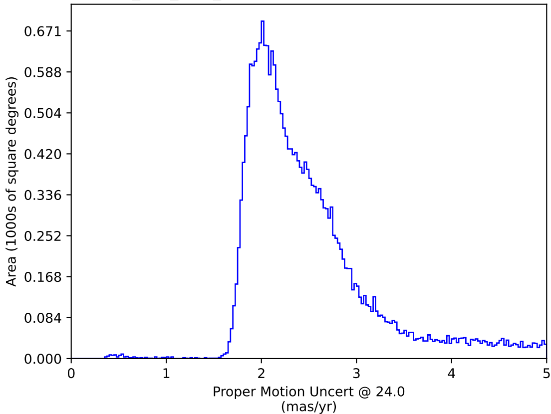
telescope_jerk_v3.5_10yrs All sky: Proper Motion Uncert @ 24.0
