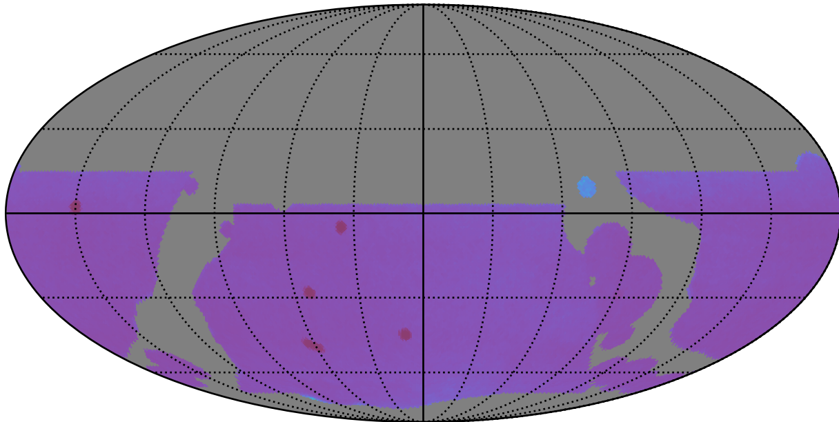
telescope_jerk_v3.5_10yrs WFD: Proper Motion Uncert @ 20.5
