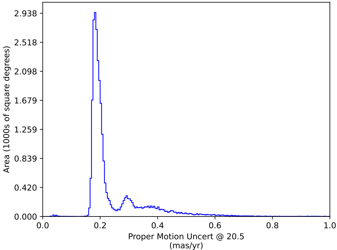
telescope_jerk_v3.5_10yrs All sky: Proper Motion Uncert @ 20.5
