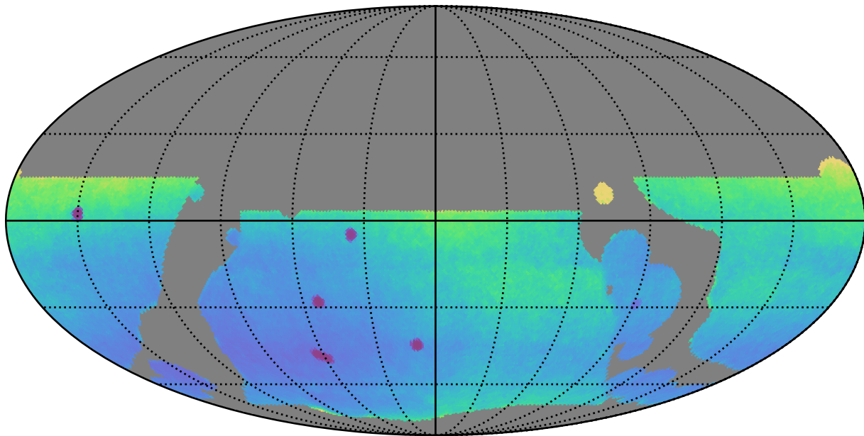
telescope_jerk_v3.5_10yrs WFD: Parallax Uncert @ 24.0
