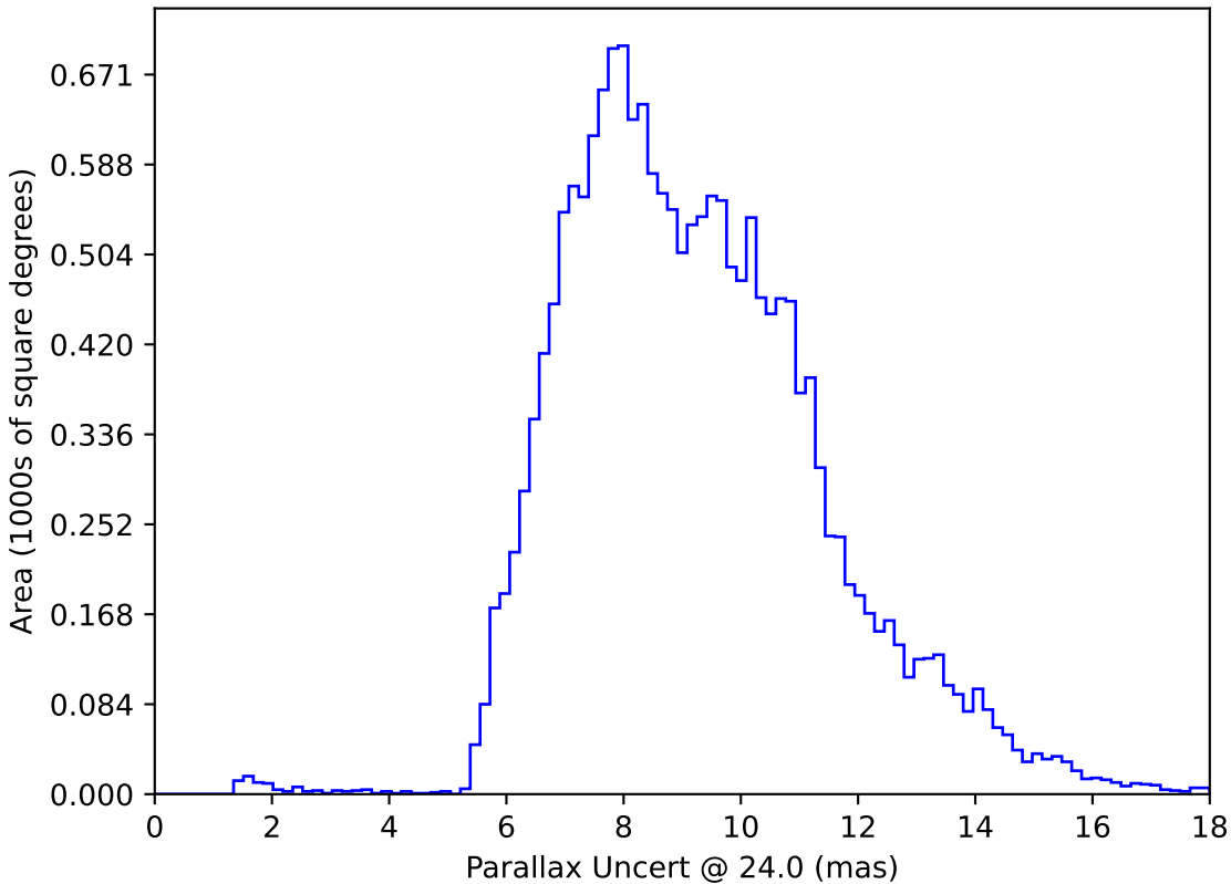
telescope_jerk_v3.5_10yrs WFD: Parallax Uncert @ 24.0
