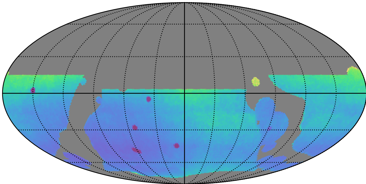
telescope_jerk_v3.5_10yrs WFD: Parallax Uncert @ 22.4
