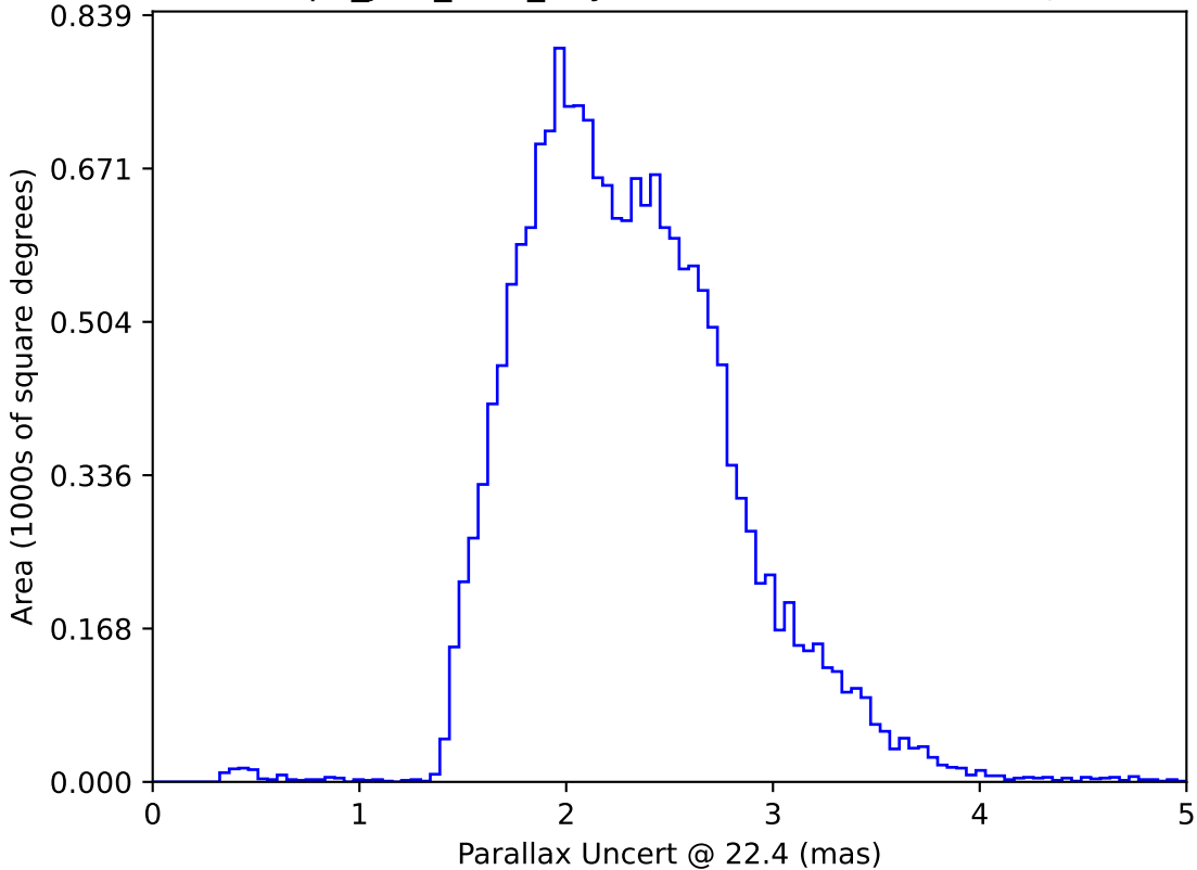
telescope_jerk_v3.5_10yrs WFD: Parallax Uncert @ 22.4
