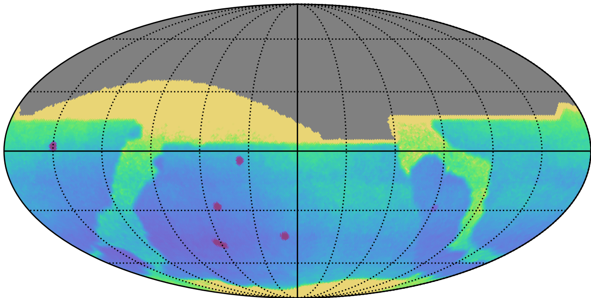
telescope_jerk_v3.5_10yrs All sky: Parallax Uncert @ 22.4
