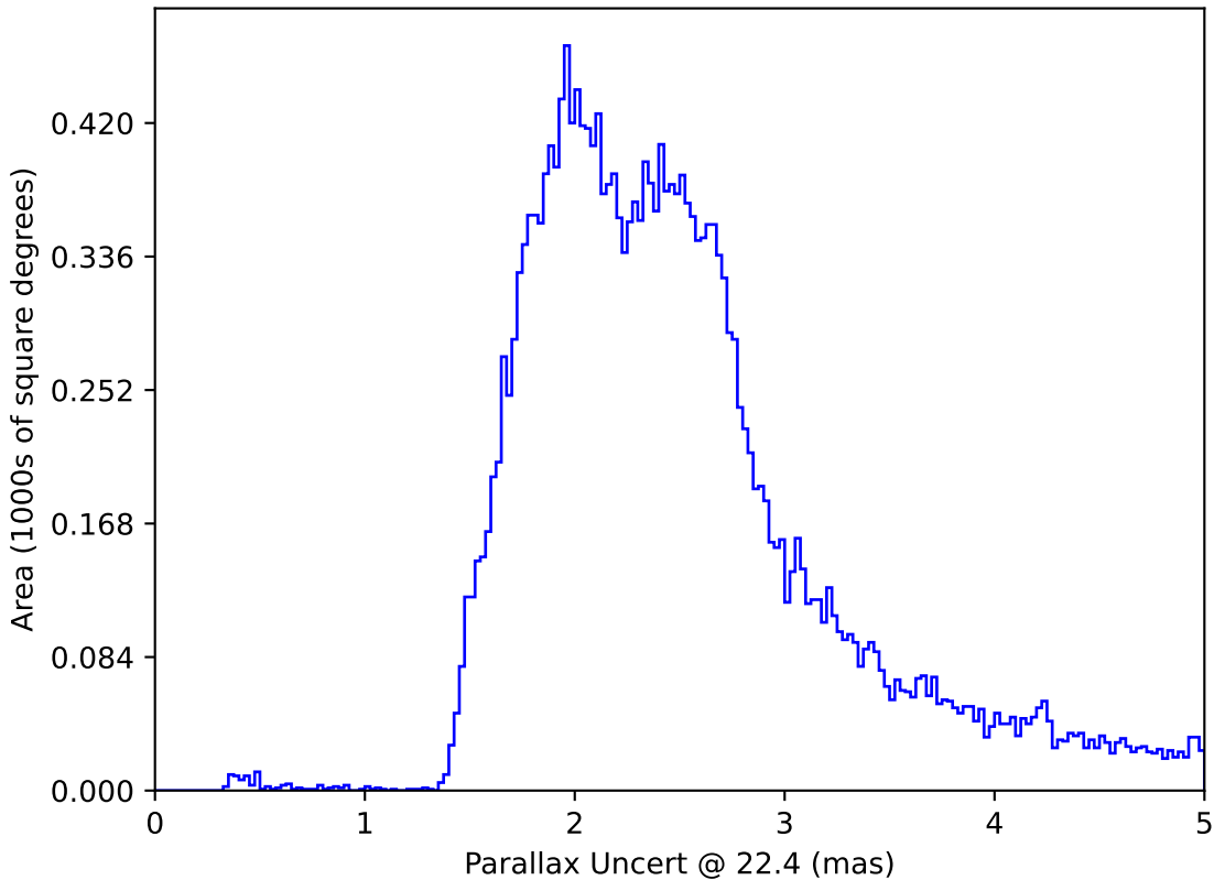
telescope_jerk_v3.5_10yrs All sky: Parallax Uncert @ 22.4
