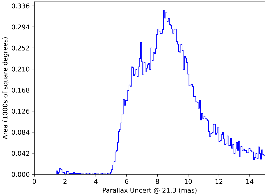
telescope_jerk_v3.5_10yrs All sky y band only: Parallax Uncert @ 21.3
