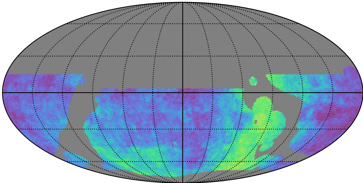
telescope_jerk_v3.5_10yrs WFD: Parallax Coverage @ 24.0
