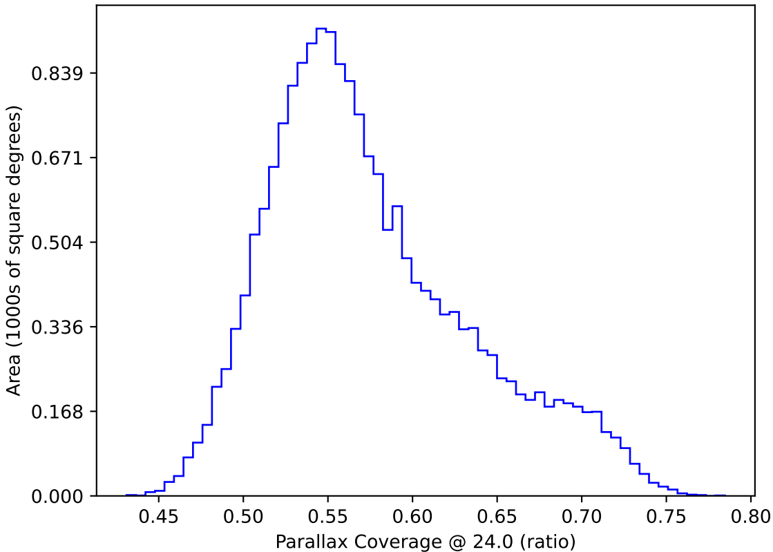
telescope_jerk_v3.5_10yrs WFD: Parallax Coverage @ 24.0
