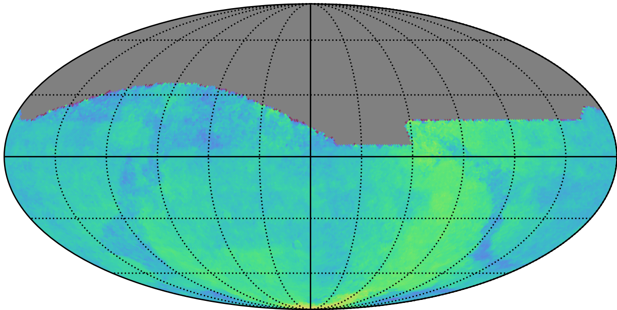
telescope_jerk_v3.5_10yrs All sky: Parallax Coverage @ 24.0
