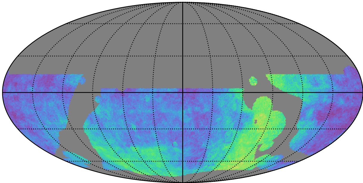
telescope_jerk_v3.5_10yrs WFD: Parallax Coverage @ 22.4
