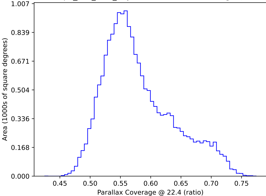
telescope_jerk_v3.5_10yrs WFD: Parallax Coverage @ 22.4
