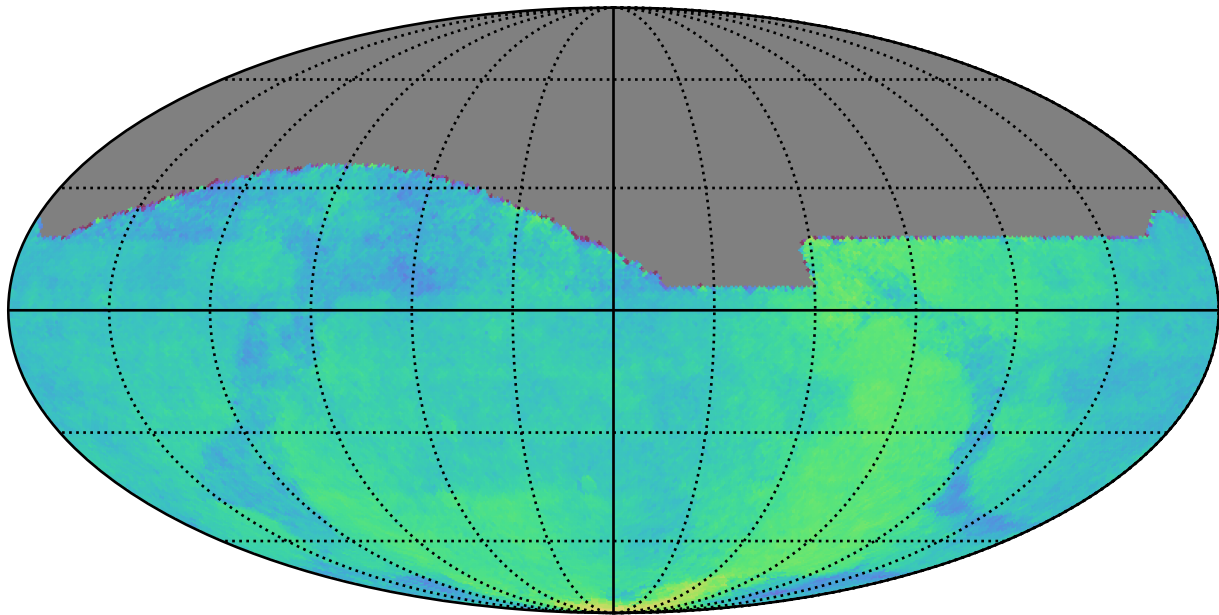
telescope_jerk_v3.5_10yrs All sky: Parallax Coverage @ 22.4
