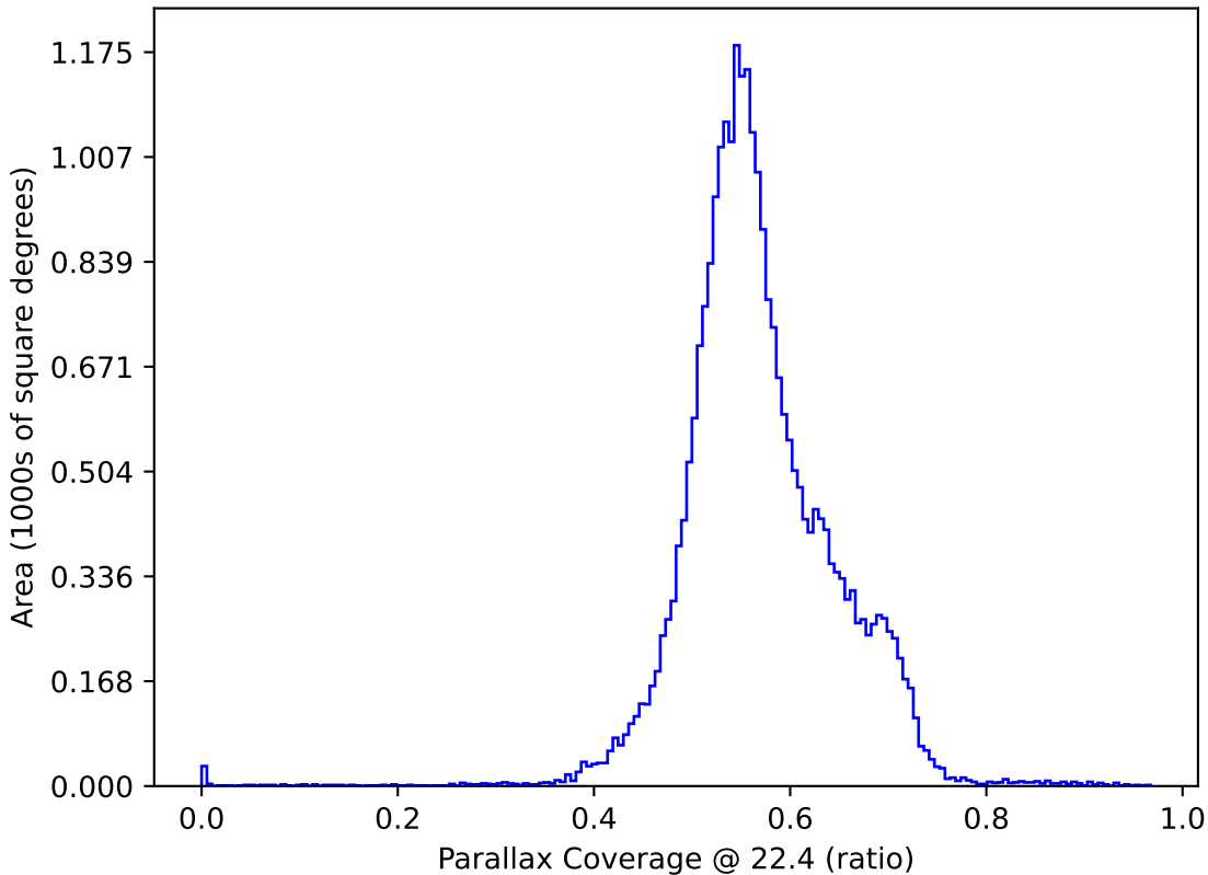
telescope_jerk_v3.5_10yrs All sky: Parallax Coverage @ 22.4
