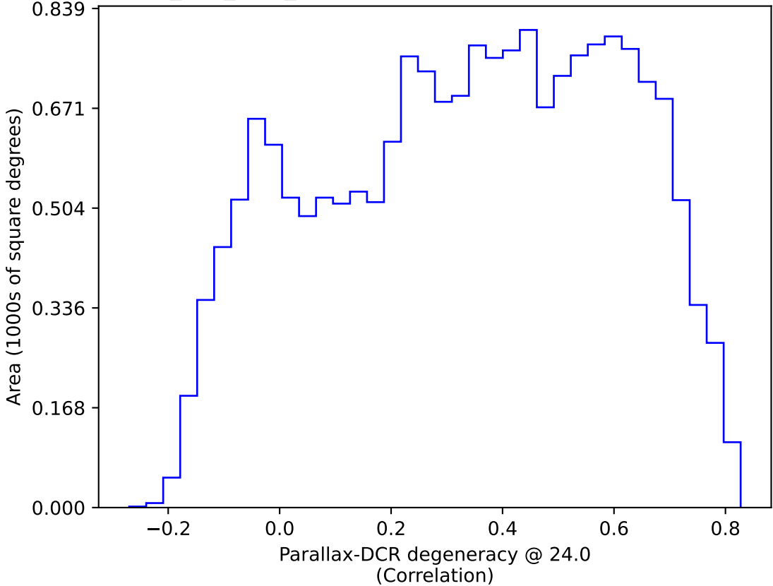
telescope_jerk_v3.5_10yrs WFD: Parallax-DCR degeneracy @ 24.0
