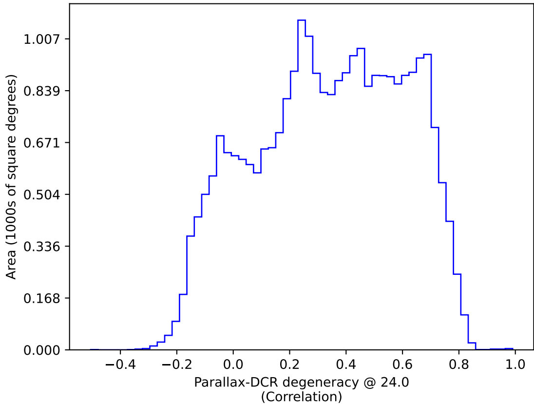
telescope_jerk_v3.5_10yrs All sky: Parallax-DCR degeneracy @ 24.0
