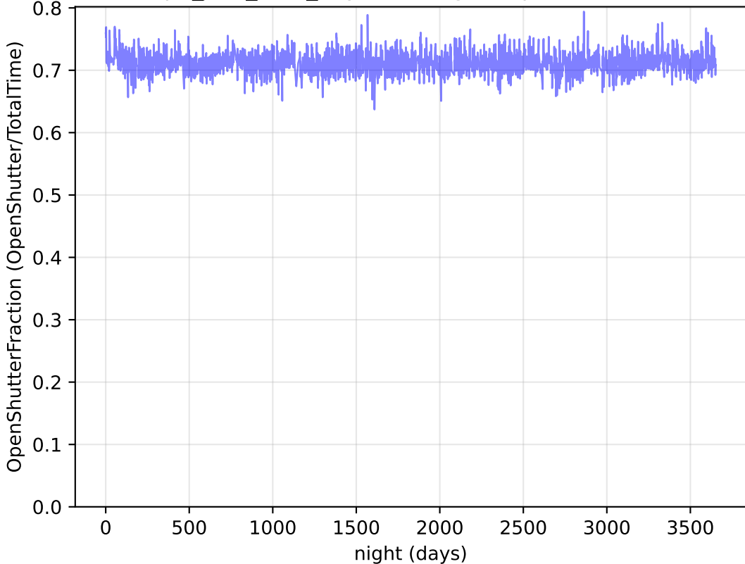
telescope_jerk_v3.5_10yrs Per night: OpenShutterFraction
