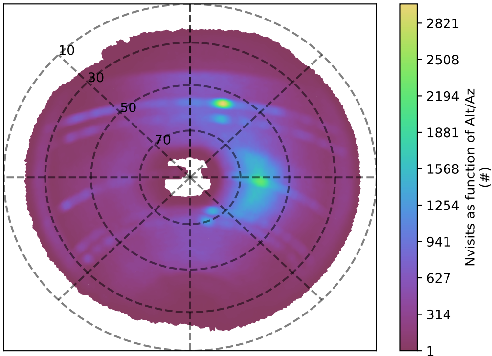
telescope_jerk_v3.5_10yrs z band: Nvisits as function of Alt/Az
