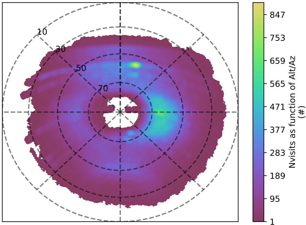
telescope_jerk_v3.5_10yrs u band: Nvisits as function of Alt/Az
