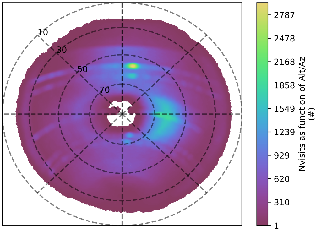
telescope_jerk_v3.5_10yrs r band: Nvisits as function of Alt/Az
