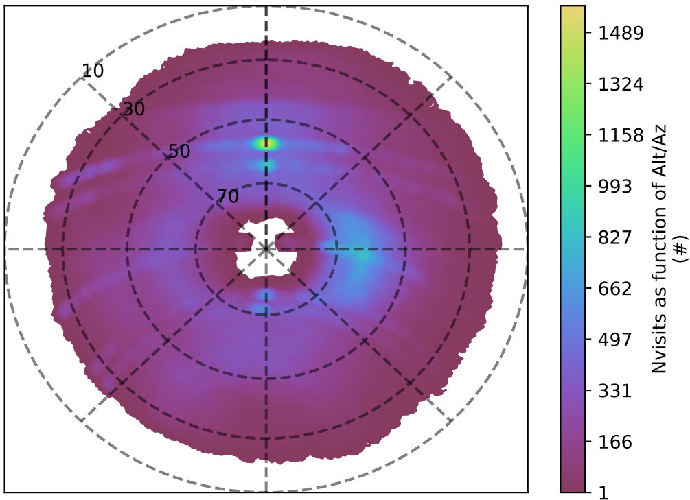
telescope_jerk_v3.5_10yrs g band: Nvisits as function of Alt/Az
