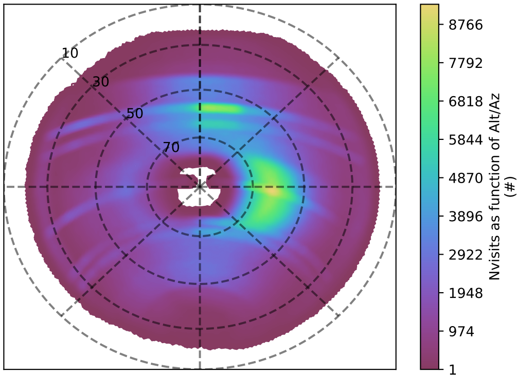
telescope_jerk_v3.5_10yrs all bands: Nvisits as function of Alt/Az
