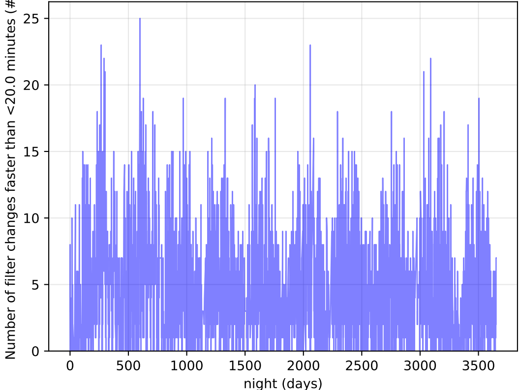
telescope_jerk_v3.5_10yrs Per Night: Number of filter changes faster than <20.0 minutes
