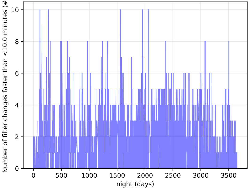
telescope_jerk_v3.5_10yrs Per Night: Number of filter changes faster than <10.0 minutes
