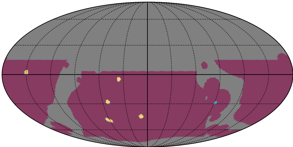
telescope_jerk_v3.5_10yrs WFD: NumberOfQuickRevisits
