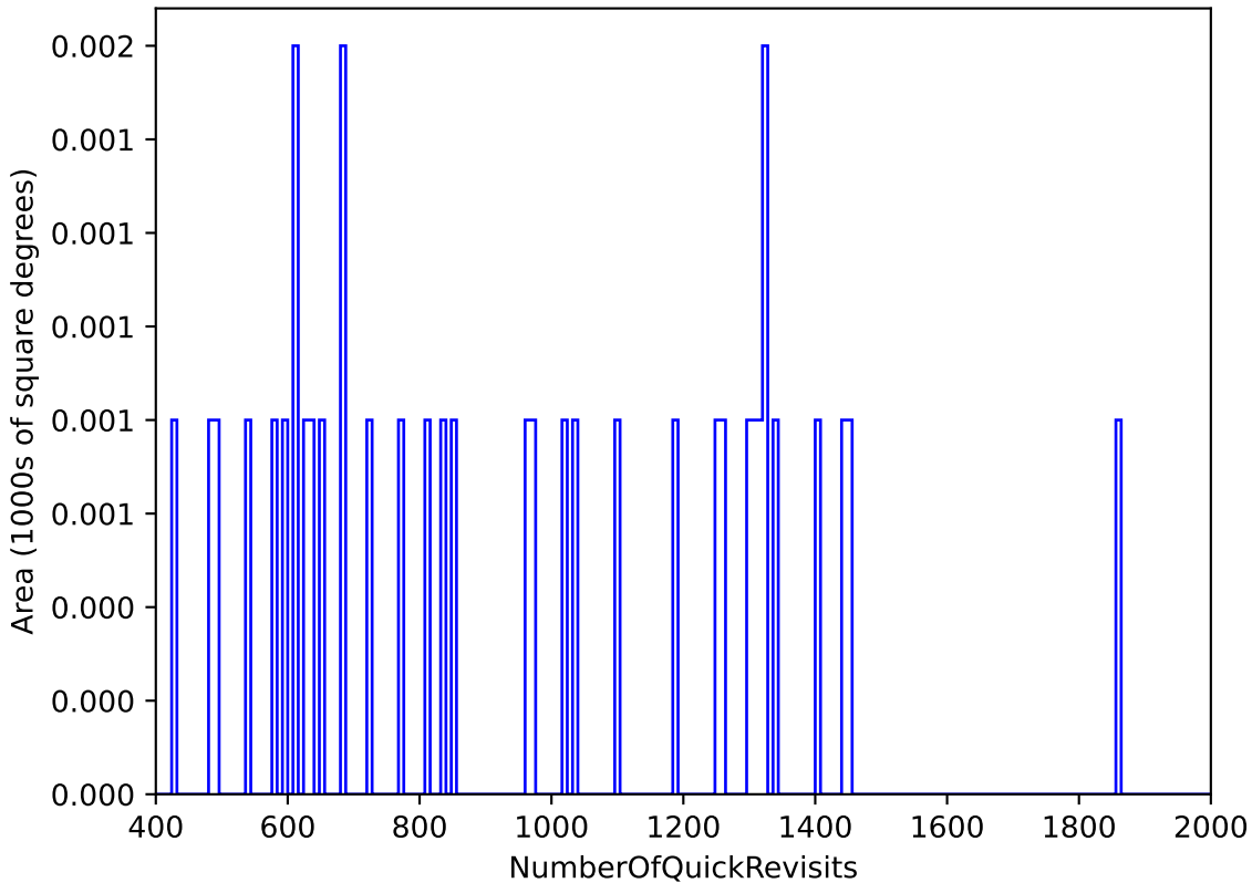
telescope_jerk_v3.5_10yrs WFD: NumberOfQuickRevisits
