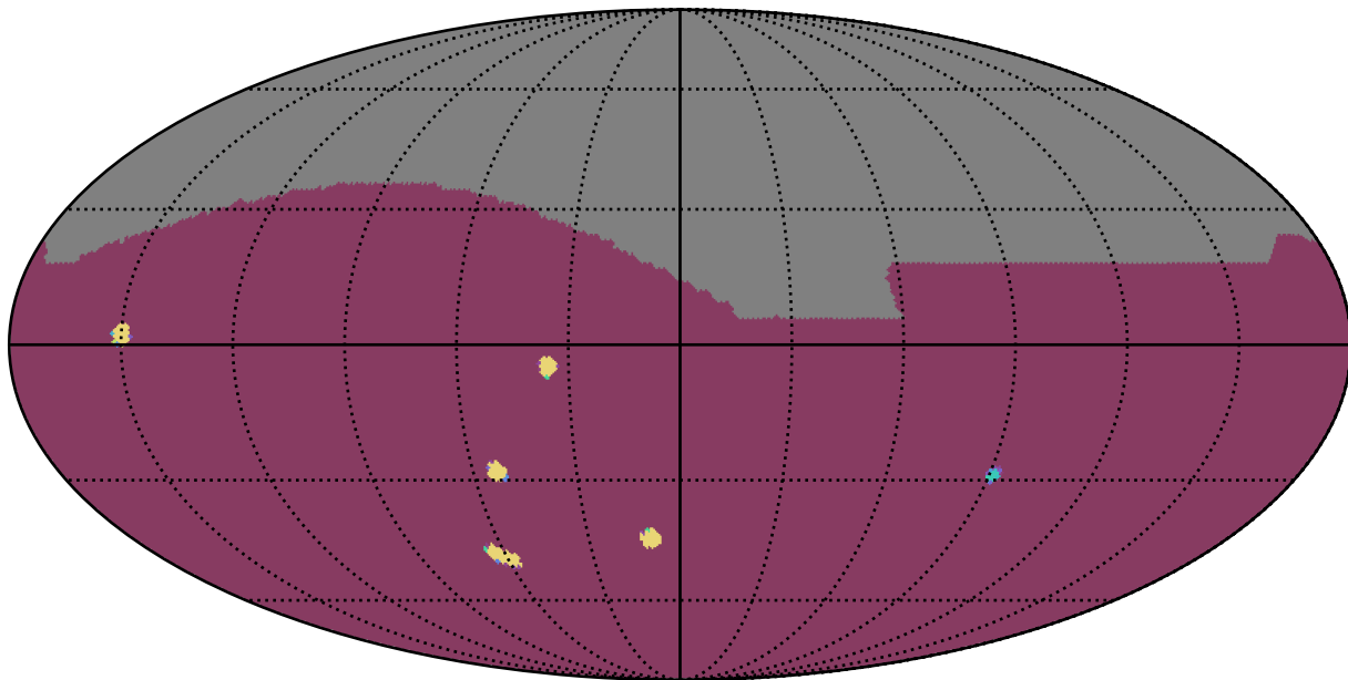
telescope_jerk_v3.5_10yrs All sky: NumberOfQuickRevisits
