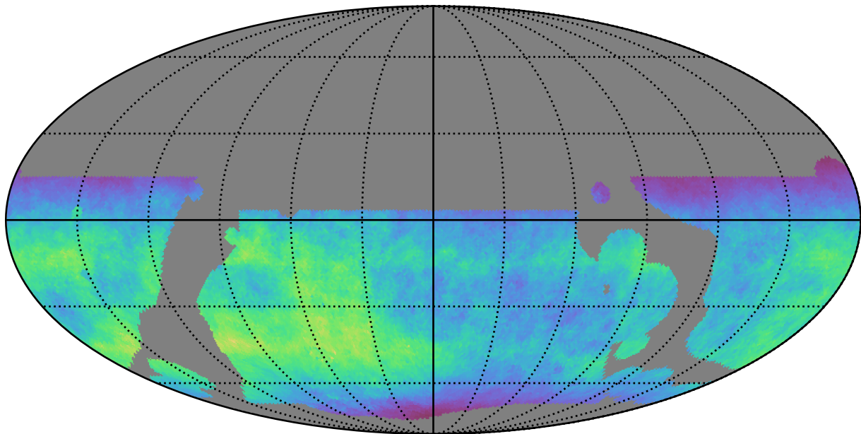
telescope_jerk_v3.5_10yrs WFD z band: Normalized Teff
