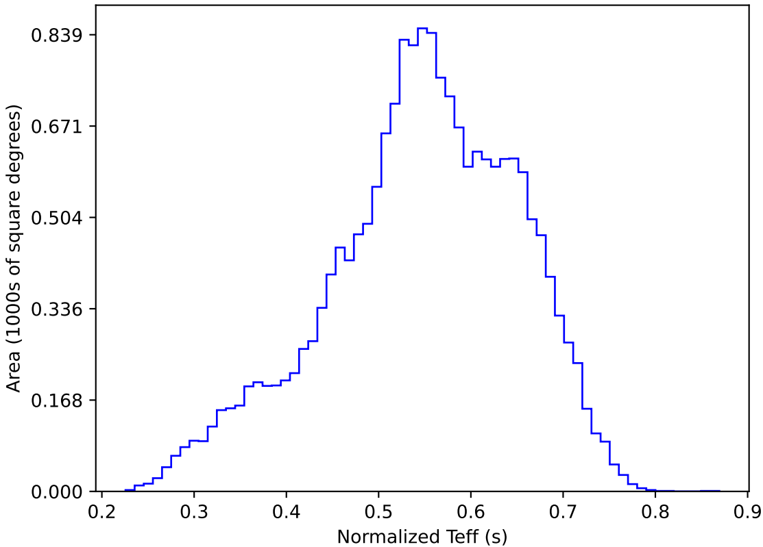
telescope_jerk_v3.5_10yrs WFD y band: Normalized Teff
