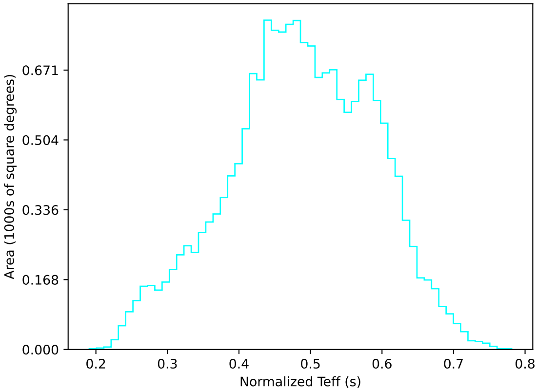
telescope_jerk_v3.5_10yrs WFD u band: Normalized Teff
