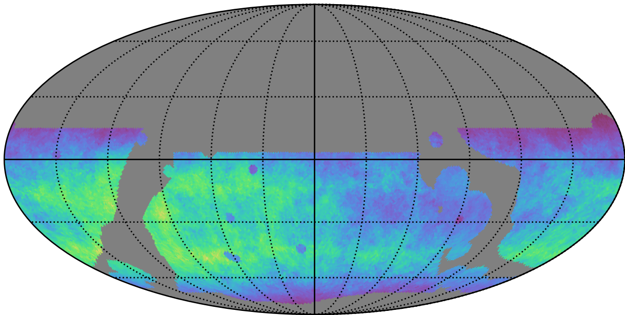
telescope_jerk_v3.5_10yrs WFD g band: Normalized Teff
